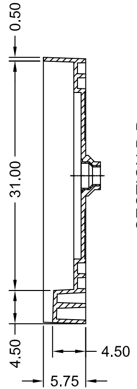
SECTION B-B
